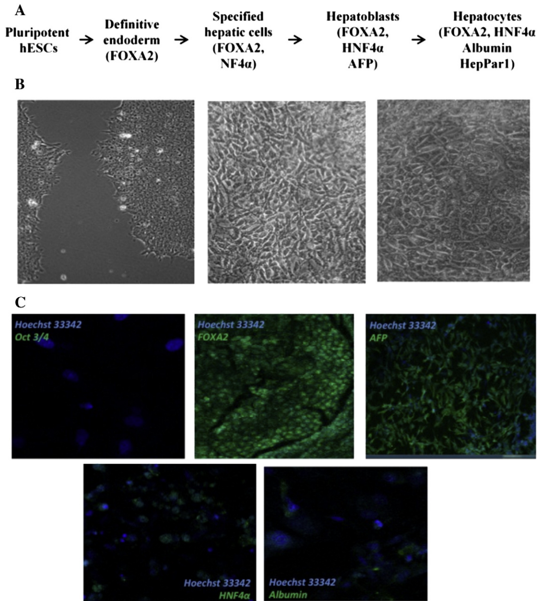
Fig. 3. Differentiation of H9 cells towards the hepatic lineage. (A) Scheme of the stages observed during differentiation of hESCs towards hepatocytes and markers expressed at each stage. (B) Cell types observed during differentiation of H9 cells during differentiation towards hepatocytes: pluripotent H9 cells (left), cells resembling premature hepatocytes (middle), cells resembling mature hepatocytes (right). (C) Expression of hepatic markers during differentiation of H9 cells detected by immunocytochemistry.
