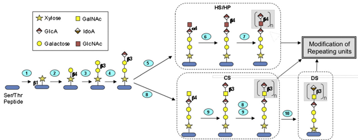
Fig. 5. Graphic diagram of GAG core tetrasaccharide biosynthesis and HS chain polymerization. The Ser/Thr-containing polypeptide core protein is glycosylated and modified through ten enzymatic reactions occurring in the endoplasmic reticulum and Golgi. Numbered steps correspond to the reactions catalyzed by the following genes (1): XYLT1 , XYLT2 , (2): B4GALT7 , (3): B3GALT6 , (4): B3GALT3 , (5): EXTL2 , EXTL3 , (6): EXT1 , EXT2 , (7): EXT1 , EXT2 , EXTL1 , EXTL3 , (8): CSGALNACT1 , CSGALNACT2 , (9): CHSY1 , CHPF1 , CHSY3 , CHPF2 , and (10): DSE1 , DSE2 .
