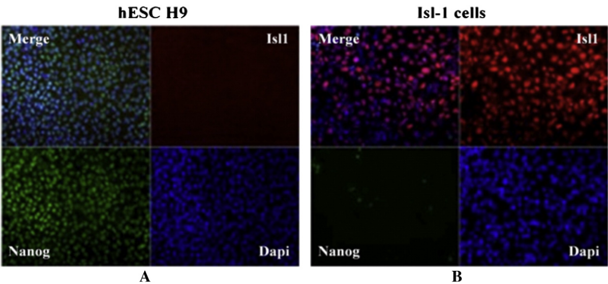
Fig. 2. Differentiation of H9 cells towards splanchnic mesoderm cells is confirmed by (A) decreased expression of Nanog and (B) an increase in the level of Isl protein.
