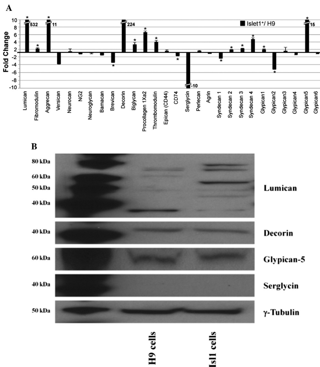
Fig. 4. Gene transcript and protein expression of GAG core proteins in H9 and splanchnic mesoderm cells. (A) Fold change of CS/DS and HS/HP core proteins detected by qRT-PCR and normalized to RPL4 . The center line indicates a value of 1 (no fold-change). Positive fold change values indicate that the transcript for a given gene is more abundant in the differentiated Isl1 + cells than in H9 cells, while negative fold change indicates that the transcript is more abundant in the undifferentiated H9 cells than the differentiated population. An asterisk (*) indicates a statistically significant change ( p < 0.05 ). Hash marks are used to indicate an off-scale value and the fold change is indicated beside the histogram bar. (B) Change in protein expression level of lumican, decorin, glypican-5 and serglycin in hESC line H9 and splanchnic mesoderm cells by Western blotting. The lane on the left shows molecular weight standards.
