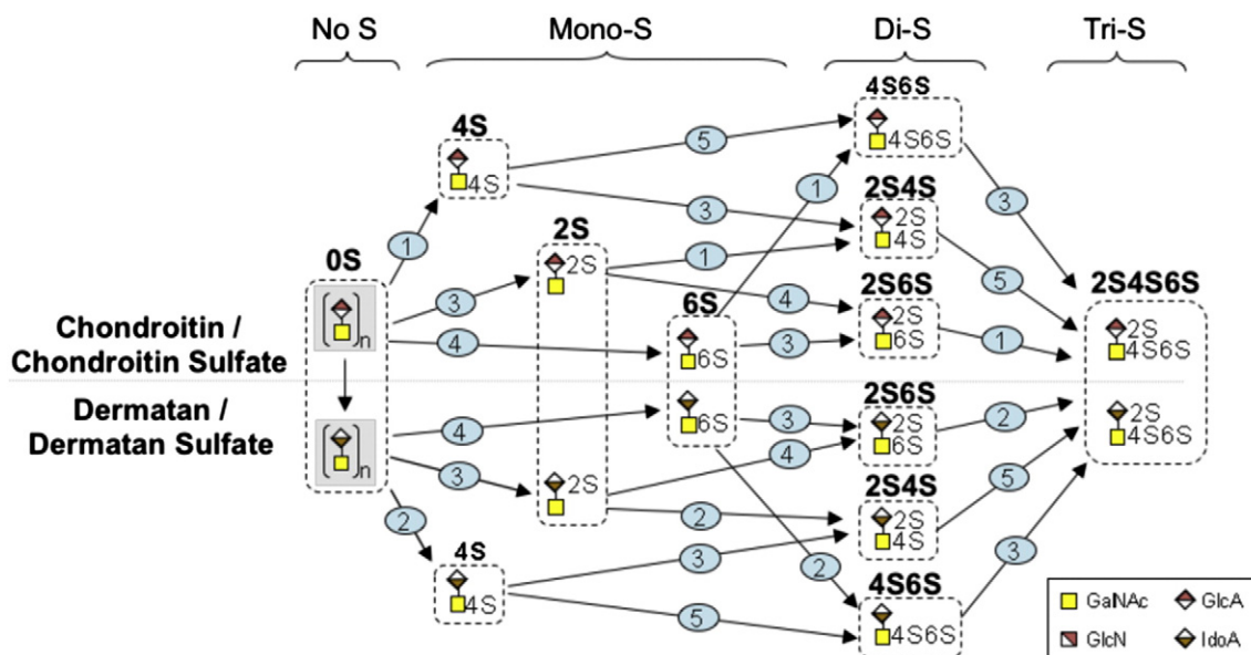
Fig. 7. Graphic diagram of the modification of the repeating units in the CS/DS chain. Numbers on steps correspond to the reactions catalyzed by enzymes encoded by the following genes (1): CHST11 , CHST12 , (2): D4ST1 , (3): UST , (4): CHST3 , CHST7 , and (5): CHST15 . The figure includes all permutations that are possible to achieve the final product, CS/DS.
