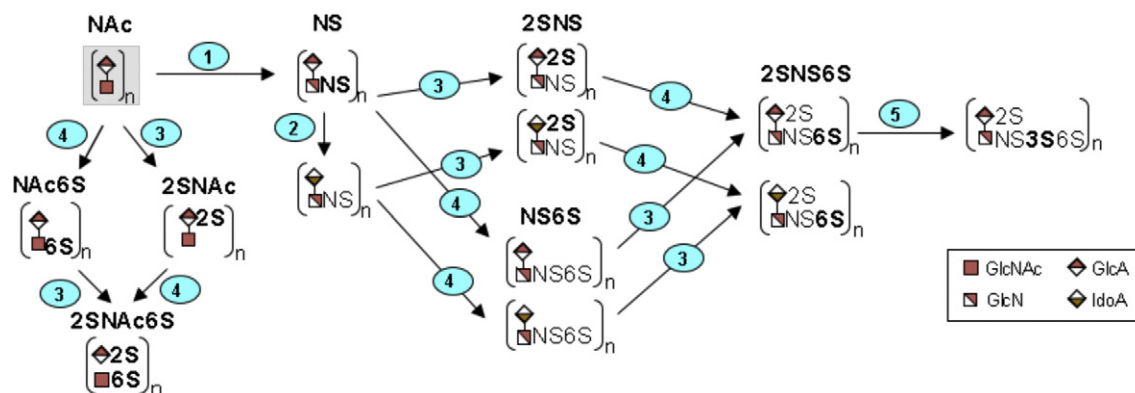
Fig. 6. Graphic diagram of the modification of the repeating units in the HS/HP chain. Numbers on steps correspond to the reactions catalyzed by enzymes encoded by the following genes (1): NDST1 , NDST2 , NDST3 , NDST4 , (2): GLCE , (3): HST2T1 , (4): HS6ST1 , HS6ST2 , HS6ST3 , and (5): HS3ST1 , HS3ST2 , HS3ST3A1 , HS3ST3B1 , HS3ST4 , HS3ST5 , HS3ST6 . While the initial, unsulfated substrate is believed to be modified by enzymes 1–5, in that order, the figure includes all other permutations that are possible to achieve the final product, HP/HS.
