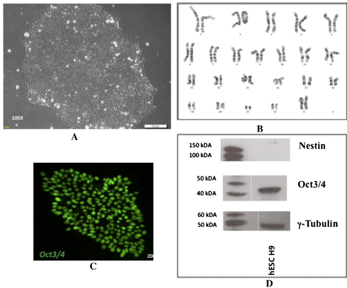
Fig. 1. Expression of pluripotency markers and karyotyping of hESC cell line H9. (A) Pluripotent H9 cells express typical morphology and (B) normal karyotype when grown on Matrigel substrate with mTeSR1 media. (C) They also express the pluripotency markers Oct3/4, as detected by immunocytochemistry and (D) do not express the early differentiation marker Nestin, as detected by immunoblotting. The lanes on the left show standard proteins with their molecular weights indicated and the lanes on the right show hESC H9. Karyotyping of WA09 cells was done by Cell Line Genetics Inc., Madison, WI.
